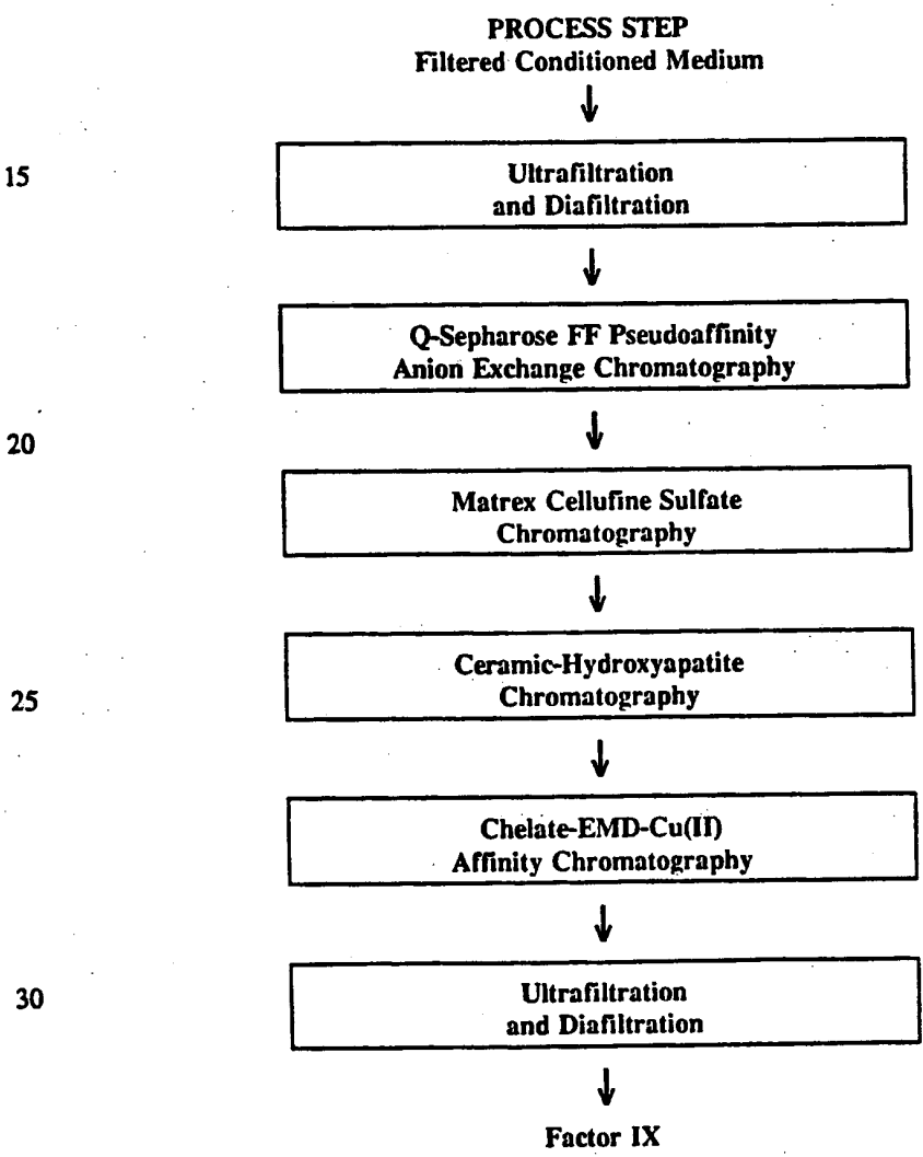
10 FIGURE 1 Overview of factor IX Purification Process
